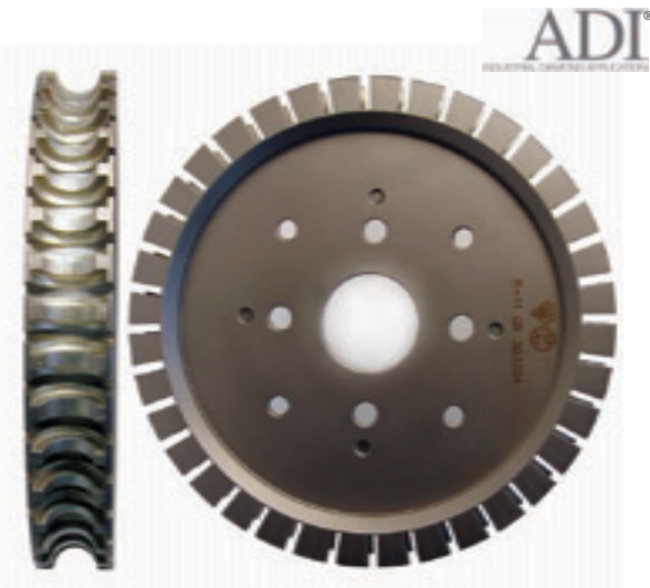
Segmented bullnose wheel O.D. 250mm, Bore 50mm
