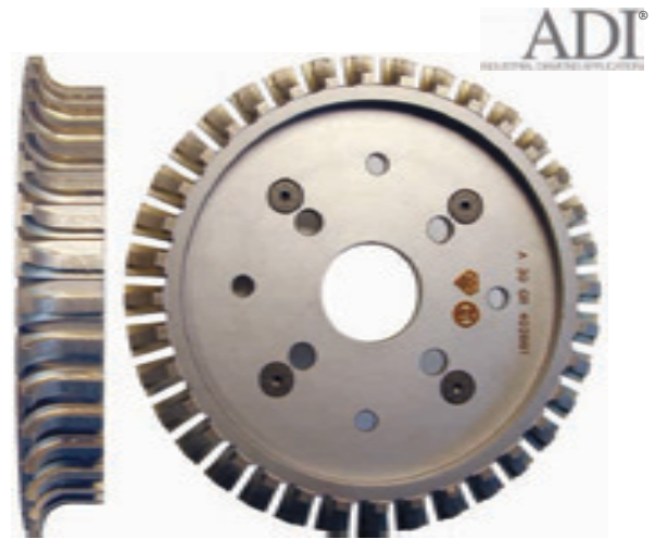
Segmented profile wheel O.D. 250mm, Bore 50mm
