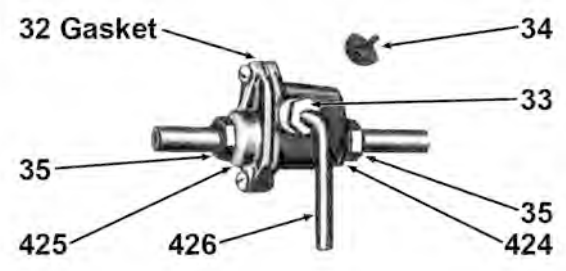
Blast Control Valve
